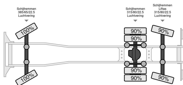
MAN TGX 26 TGX 26.470 - BDF - Retarder - 2021 - Steering axle
