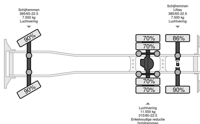
Scania R450 N333
