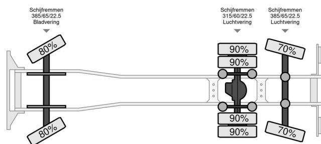
Volvo FH 480 FH 480 Cattle transport
