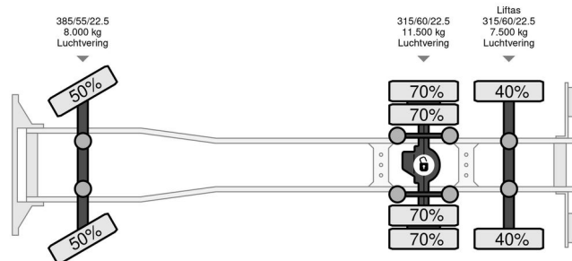
Volvo FH 500 VTJ3R
