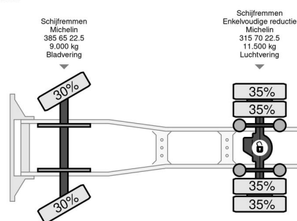
DAF XF 460 H4EN3 - 2016 - Euro 6 - Walking floor + tipper hydraulic 4x2
