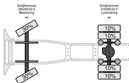
Volvo FH 16.660 FH 16.660 - 2007 - Euro 4 - Retarder
