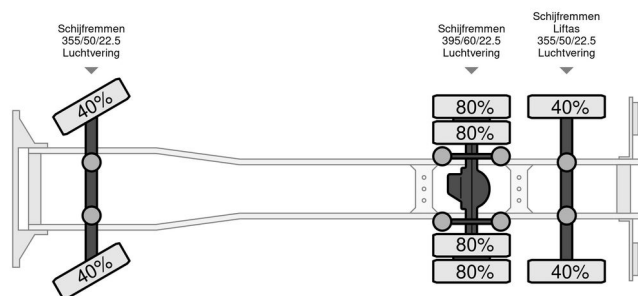
DAF XF 510 Super Space Cab
