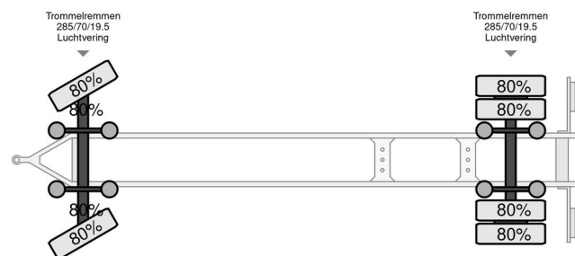
Jumbo MV200E
