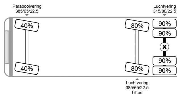
Scania R164-580 V8 R 164 GA 6x2 ...
