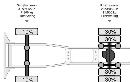
DAF XF 105.410 XF 105-410 - 2011 - Retarder
