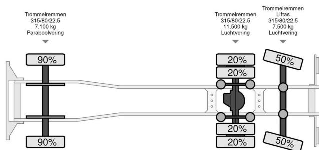
Scania R143-420 V8 EFFER 8200 Kraan - Effer 8200 Crane
