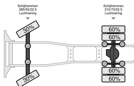
Scania R164-480 V8 Full Air!
