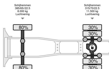
Scania S580 S580 Full air, King of the road, Show Truck! www.companjen.nl 4x2
