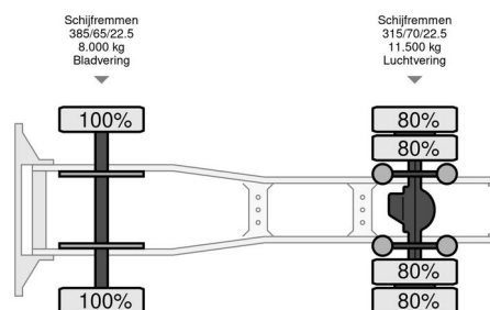
DAF XF 480 XF Super space cab
