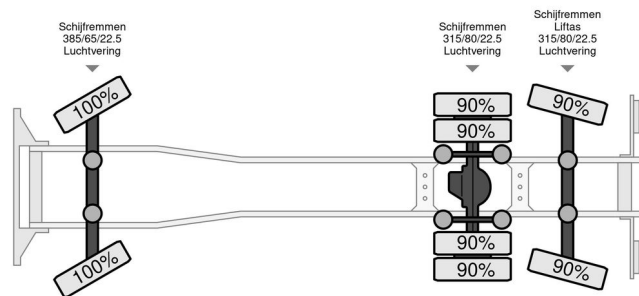
MAN TGX 26 TGX 26.470 - BDF - Retarder - 2021 - Steering axle 6x2
