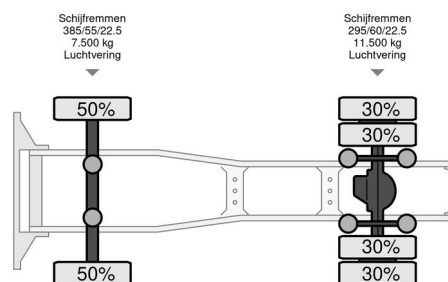
MAN TGX L 2007.46.001
