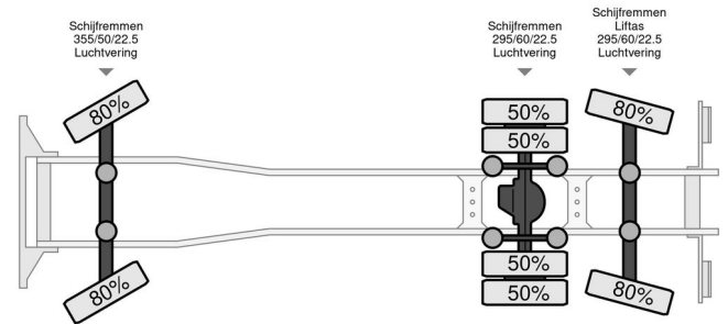
Scania R450 NGS R450
