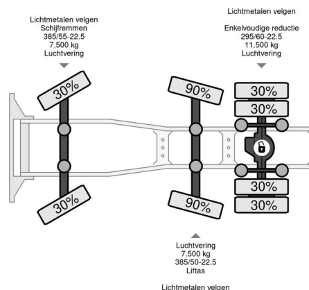
Scania R490 N330
