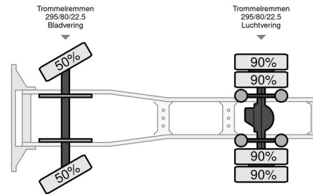
Volvo F 16.485 F16 - 485 - 1989 - Oldtimer
