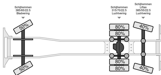
Volvo FM 9
