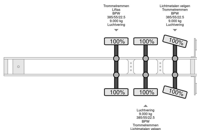
CUPPERS 3OZ4 - Motor cycle transport
