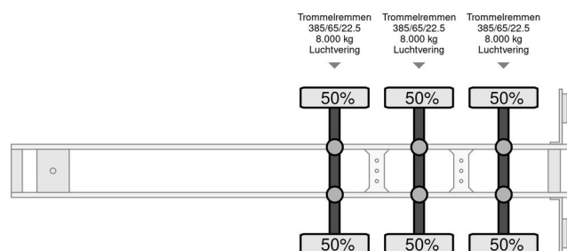
Gray and Adams Companjen Cattle Carrier - 2007 - 2 floors livestock transport
