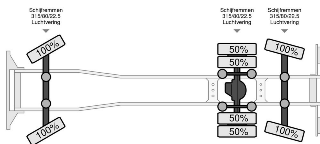
Scania R450
